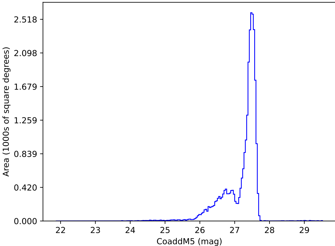
ddf_acor_sf15_lsf40_lsr10_v3.4_10yrs : CoaddM5
