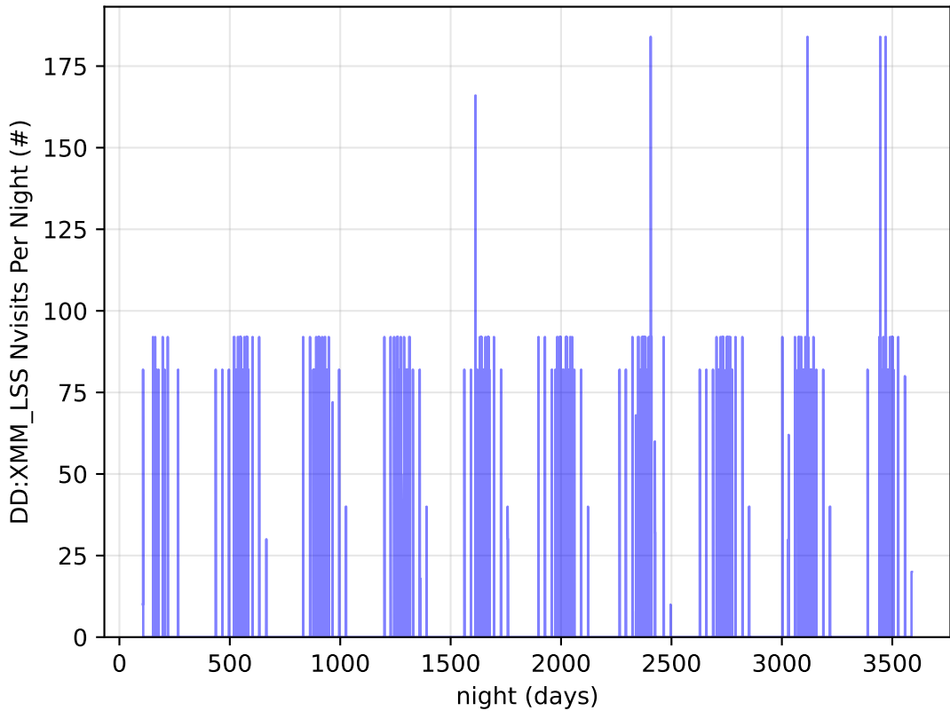
ddf_acor_sf15_lsf40_lsr10_v3.4_10yrs all bands: DD:XMM_LSS Nvisits Per Night
