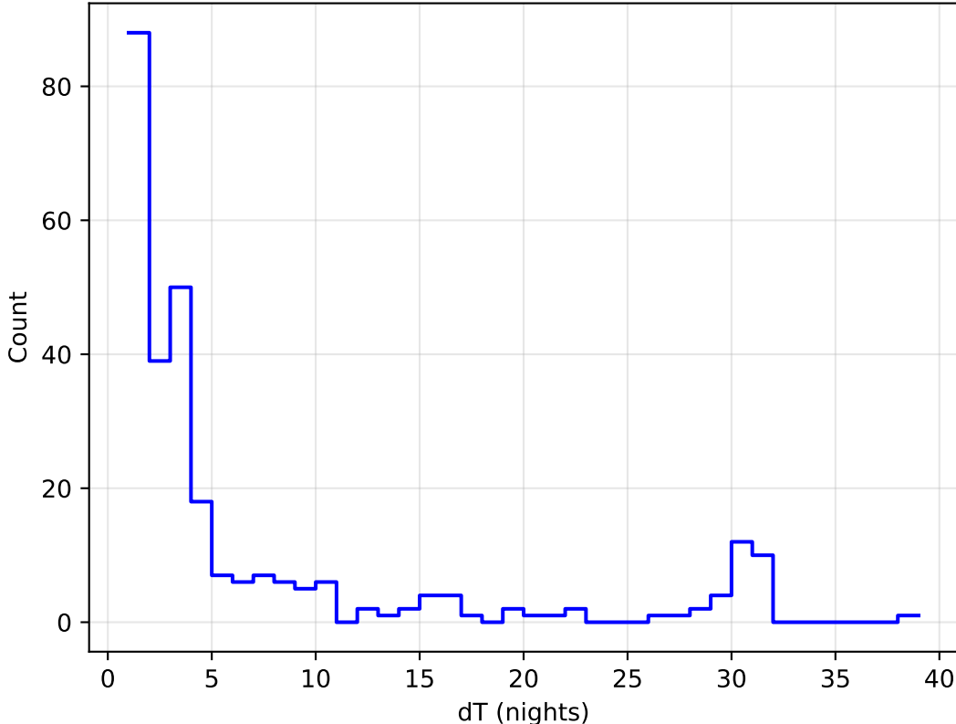
ddf_acor_sf15_lsf40_lsr10_v3.4_10yrs all bands: DD:XMM_LSS Delta Nights Histogram
