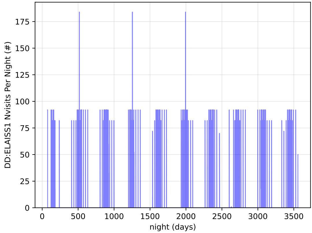
ddf_acor_sf15_lsf40_lsr10_v3.4_10yrs all bands: DD:ELAISS1 Nvisits Per Night
