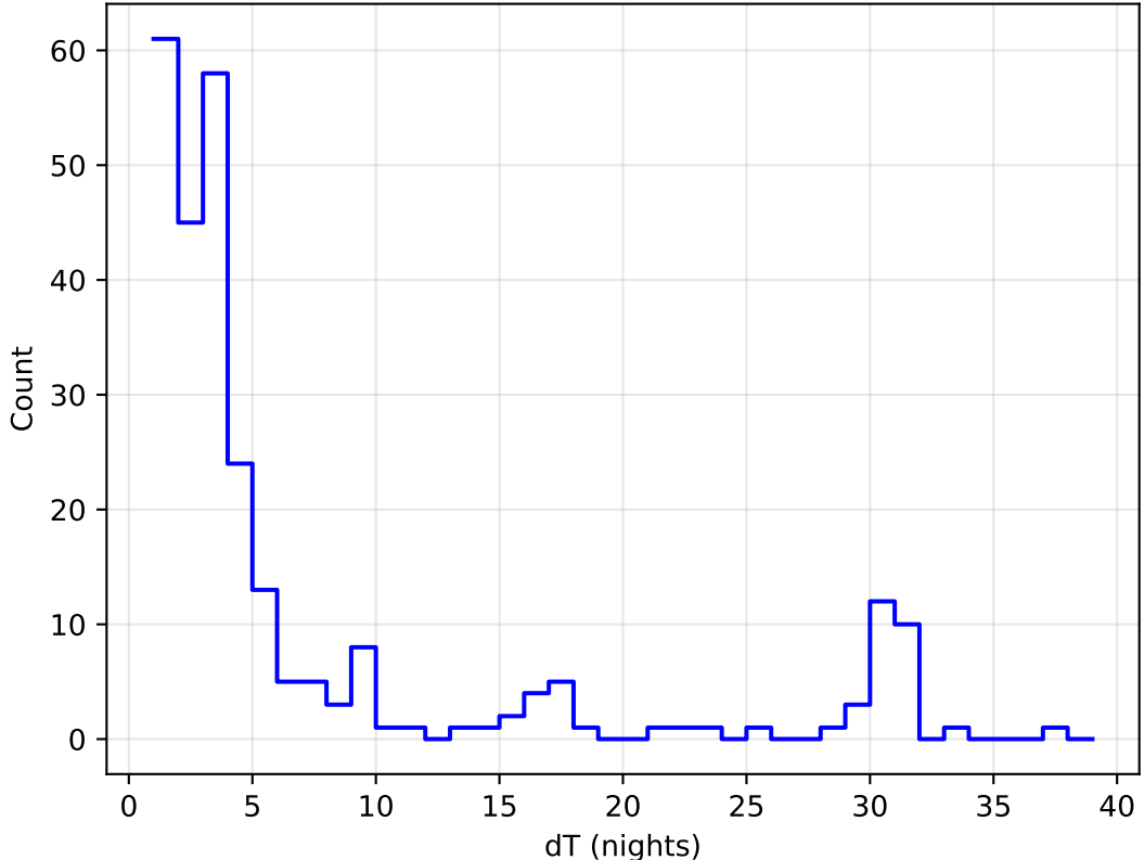
ddf_acor_sf15_lsf40_lsr10_v3.4_10yrs all bands: DD:ELAISS1 Delta Nights Histogram
