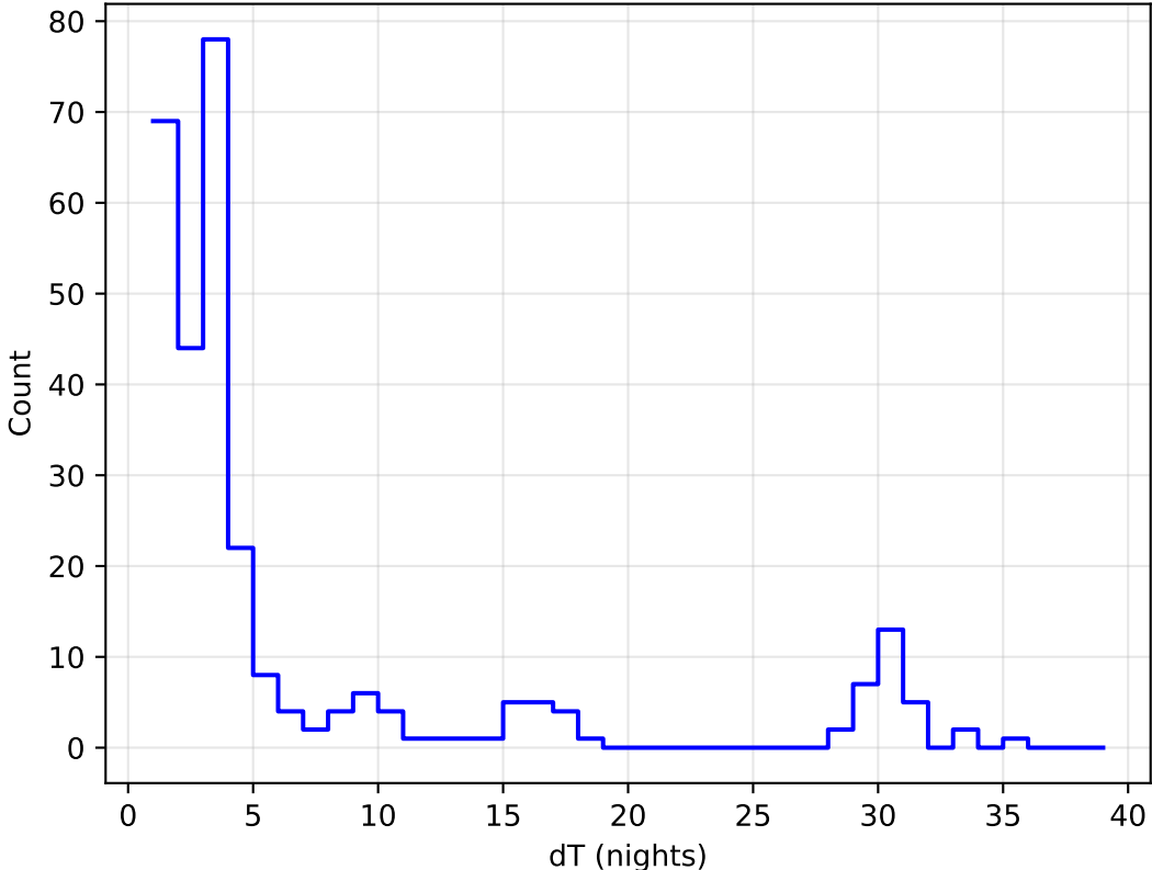
ddf_acor_sf15_lsf40_lsr10_v3.4_10yrs all bands: DD:EDFS Delta Nights Histogram
