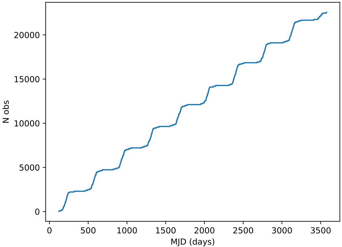
ddf_acor_sf15_lsf40_lsr10_v3.4_10yrs all bands: DD:EDFS Cumulative NVisits
