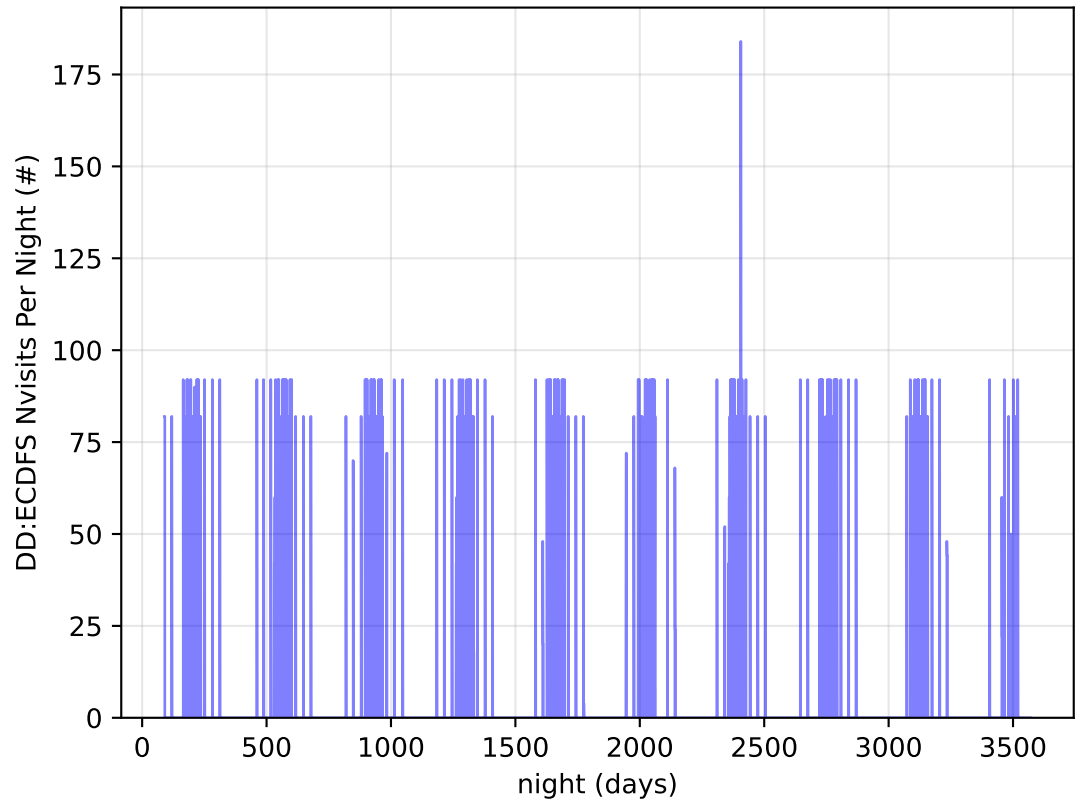
ddf_acor_sf15_lsf40_lsr10_v3.4_10yrs all bands: DD:ECDFS Nvisits Per Night
