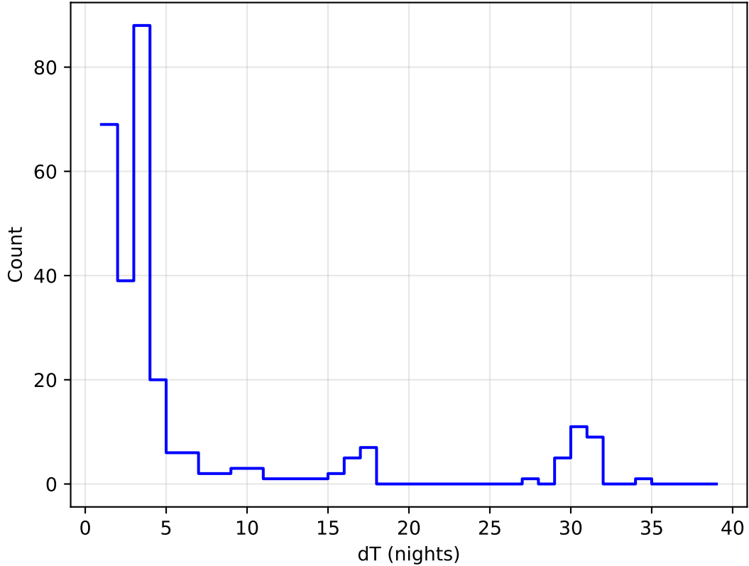
ddf_acor_sf15_lsf40_lsr10_v3.4_10yrs all bands: DD:ECDFS Delta Nights Histogram
