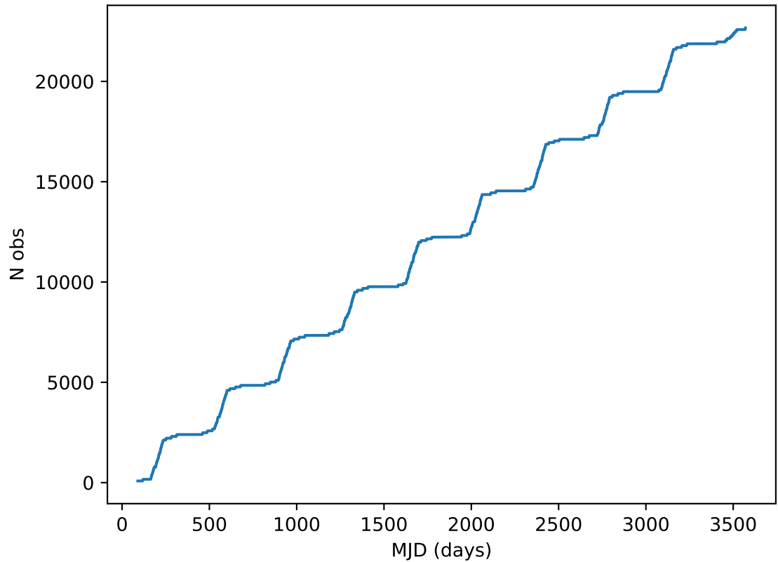
ddf_acor_sf15_lsf40_lsr10_v3.4_10yrs all bands: DD:ECDFS Cumulative NVisits
