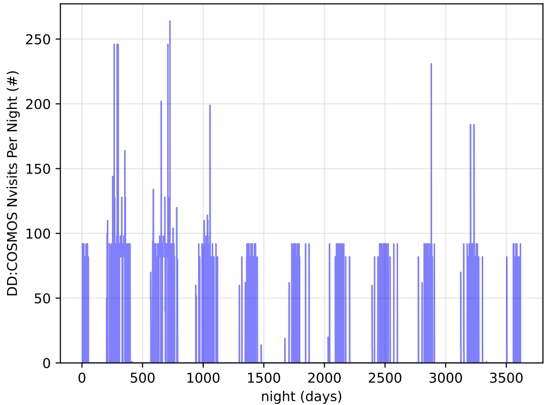
ddf_acor_sf15_lsf40_lsr10_v3.4_10yrs all bands: DD:COSMOS Nvisits Per Night
