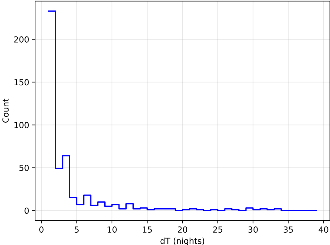
ddf_acor_sf15_Isf40_Isr10_v3.4_10yrs all bands: DD:COSMOS Delta Nights Histogram
