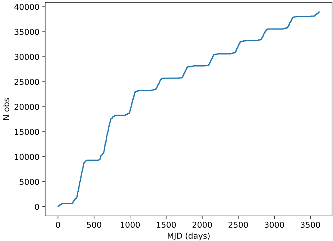
ddf_acor_sf15_lsf40_lsr10_v3.4_10yrs all bands: DD: COSMOS Cumulative NVisits
