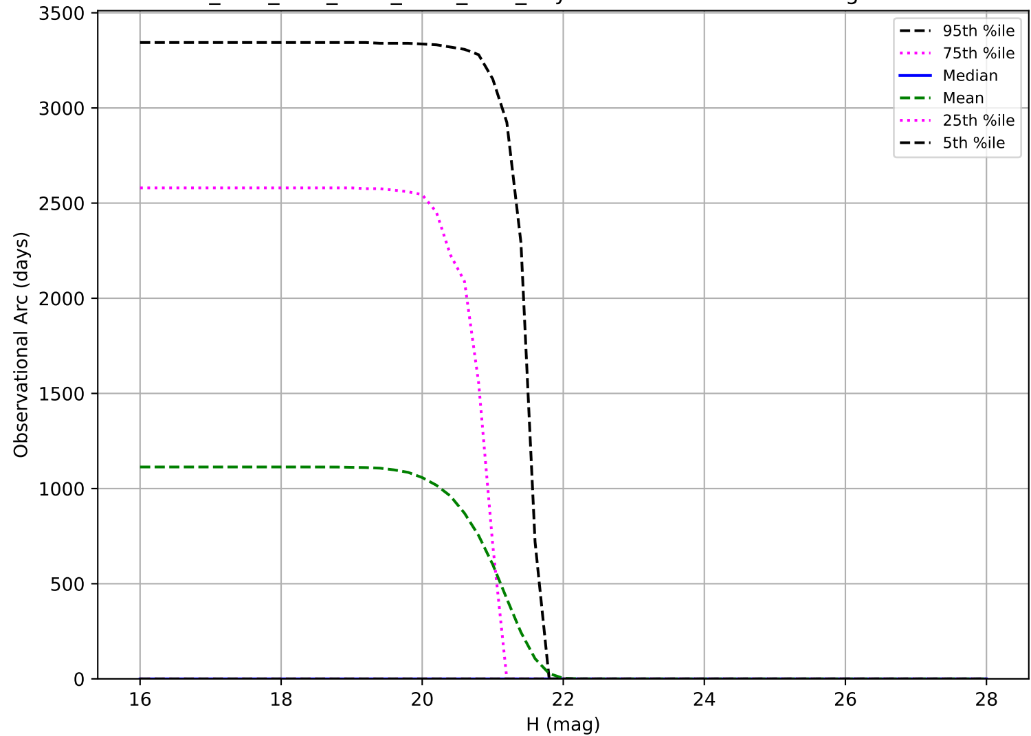
ddf_acor_sf15_lsf30_lsr50_v3.4_10yrs: Observational Arc Length Vatira
