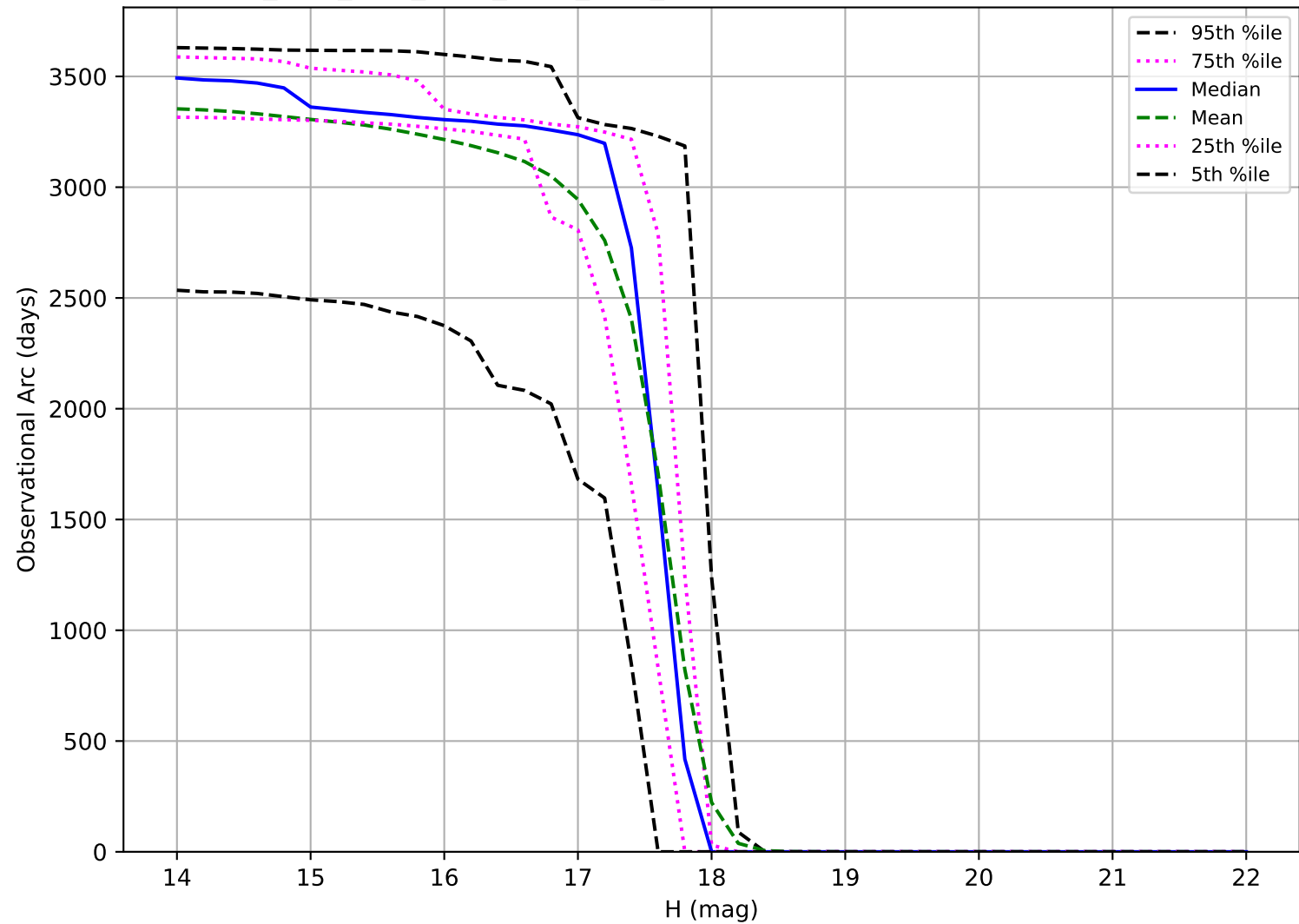
ddf_acor_sf15_lsf30_lsr50_v3.4_10yrs: Observational Arc Length Trojan
