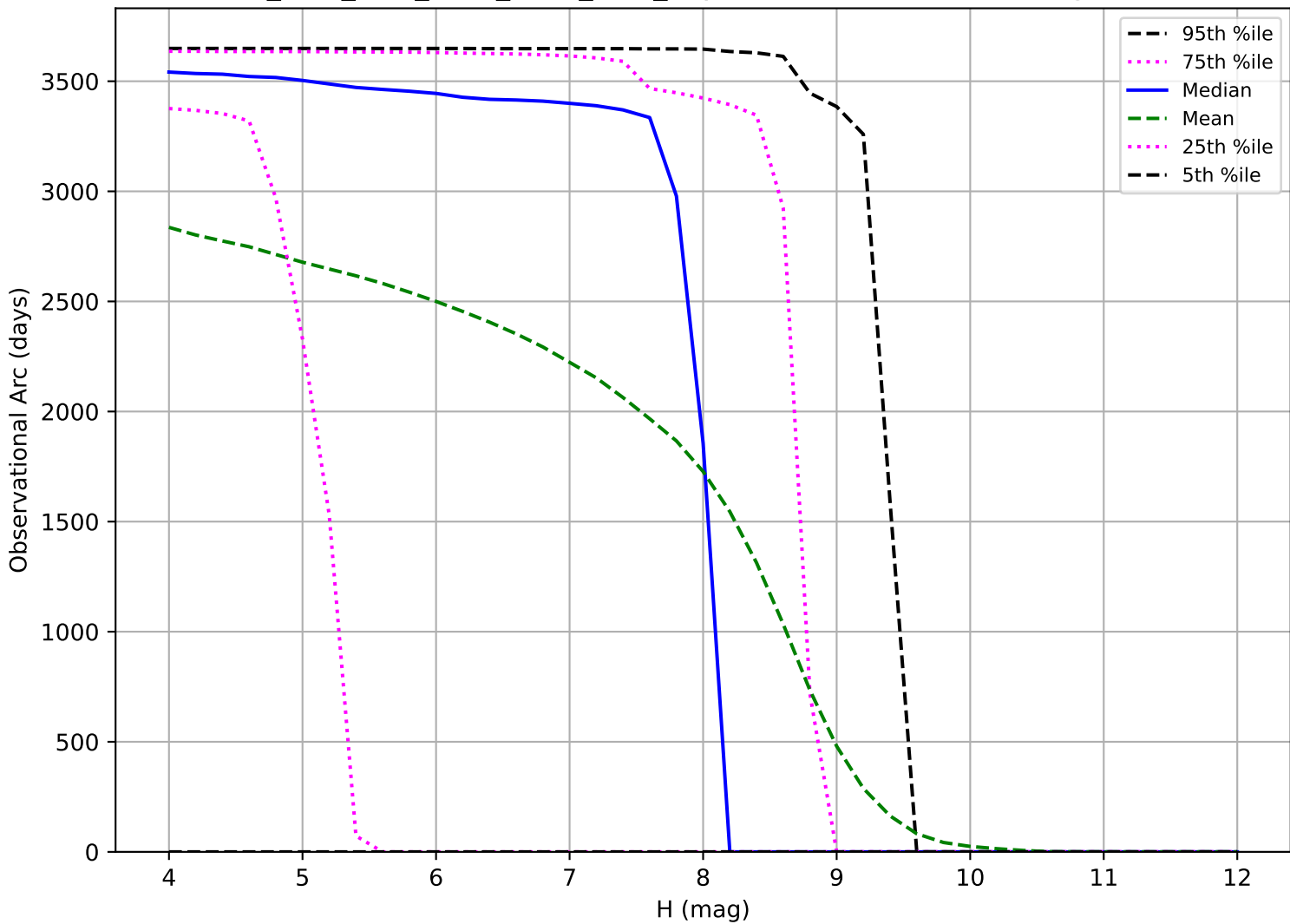
ddf_acor_sf15_Isf30_Isr50_v3.4_10yrs: Observational Arc Length TNO
