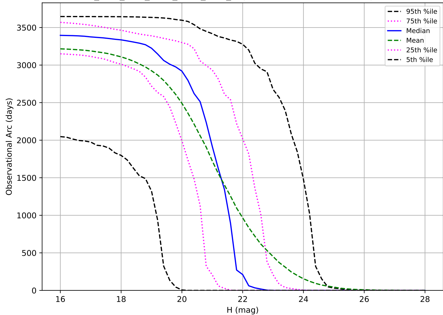
ddf_acor_sf15_lsf30_lsr50_v3.4_10yrs: Observational Arc Length PHA
