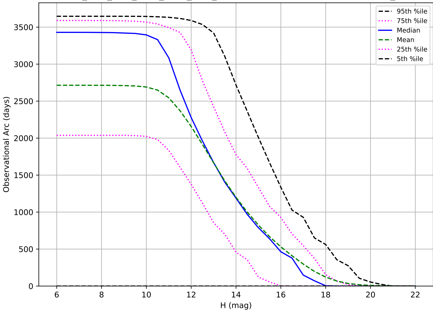
ddf_acor_sf15_lsf30_lsr50_v3.4_10yrs: Observational Arc Length OCC_r5
