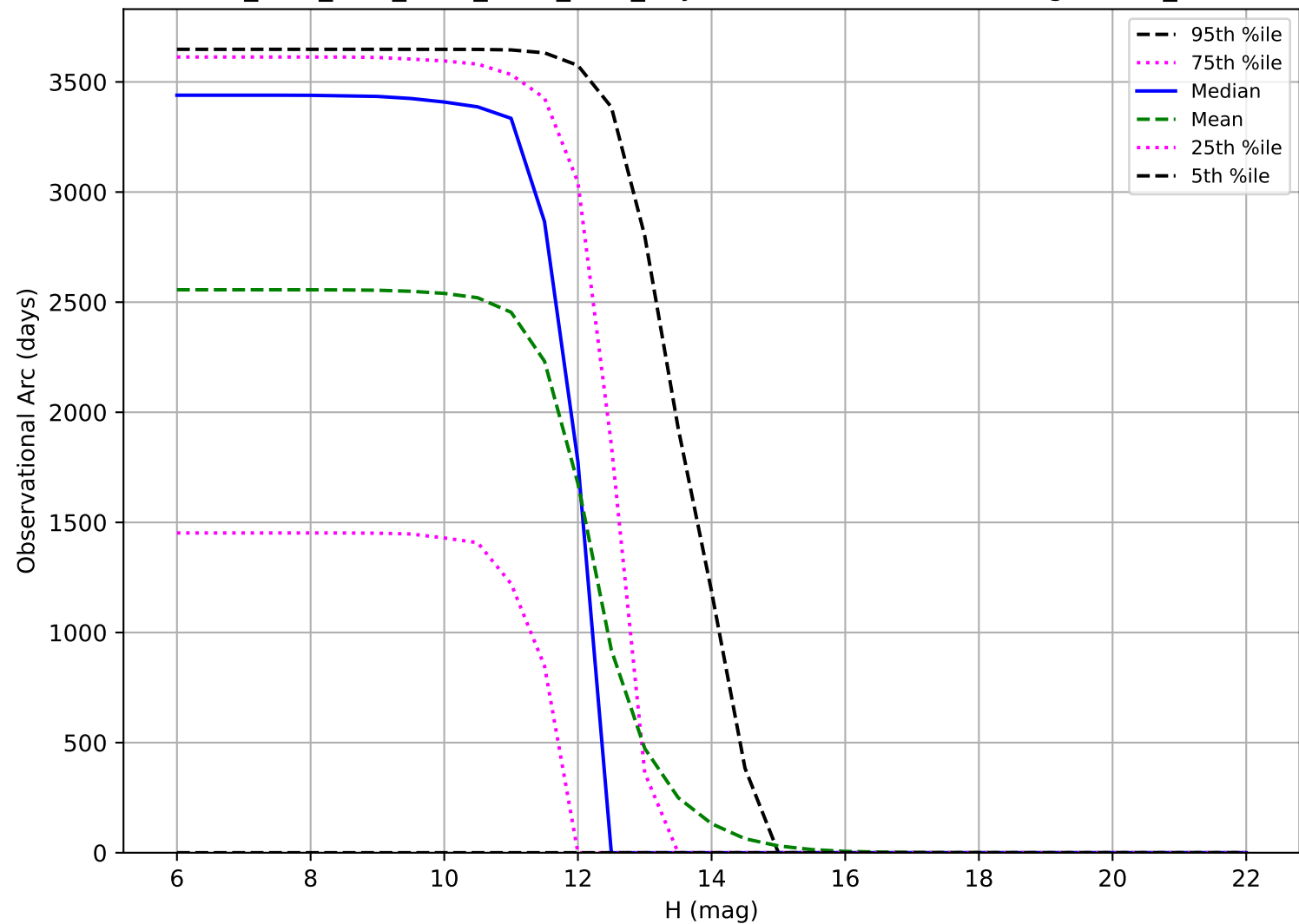
ddf_acor_sf15_lsf30_lsr50_v3.4_10yrs: Observational Arc Length OCC_r20
