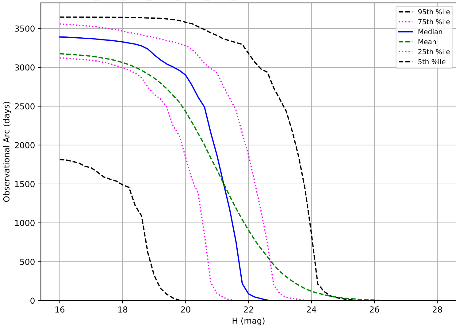
ddf_acor_sf15_lsf30_lsr50_v3.4_10yrs: Observational Arc Length NEO
