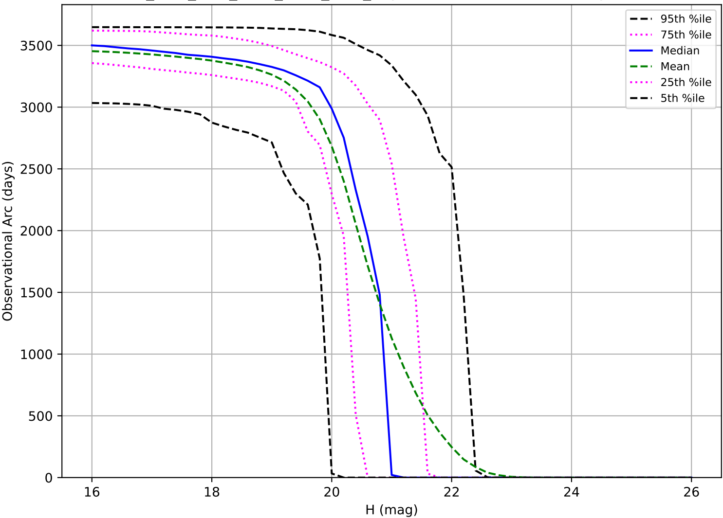
ddf_acor_sf15_lsf30_lsr50_v3.4_10yrs: Observational Arc Length MBA
