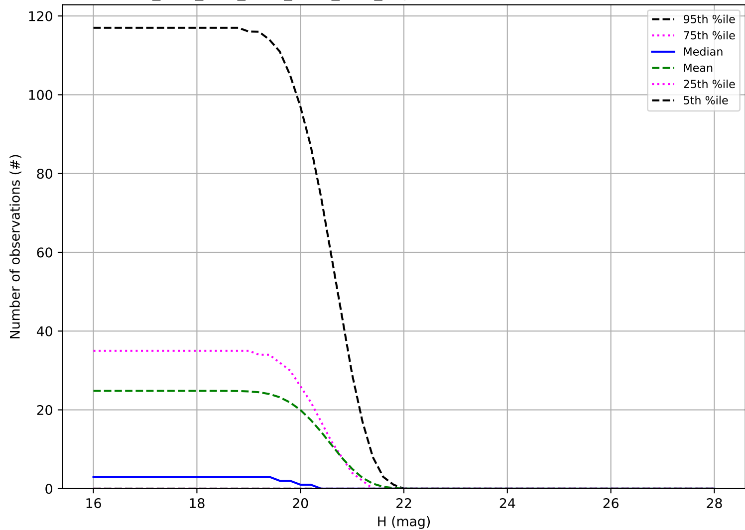
ddf_acor_sf15_lsf30_lsr50_v3.4_10yrs: Number of observations Vatira
