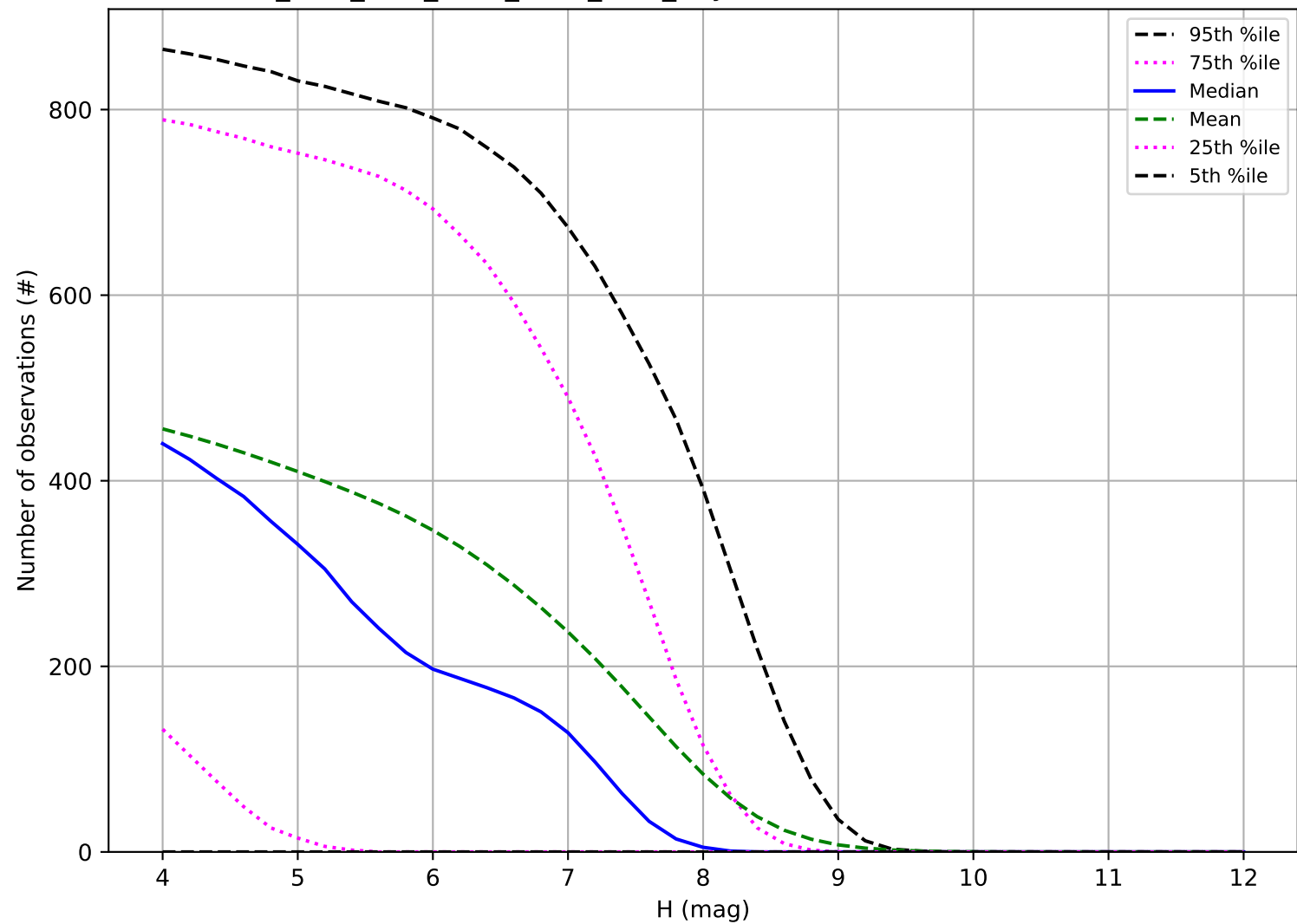
ddf_acor_sf15_lsf30_lsr50_v3.4_10yrs: Number of observations TNO
