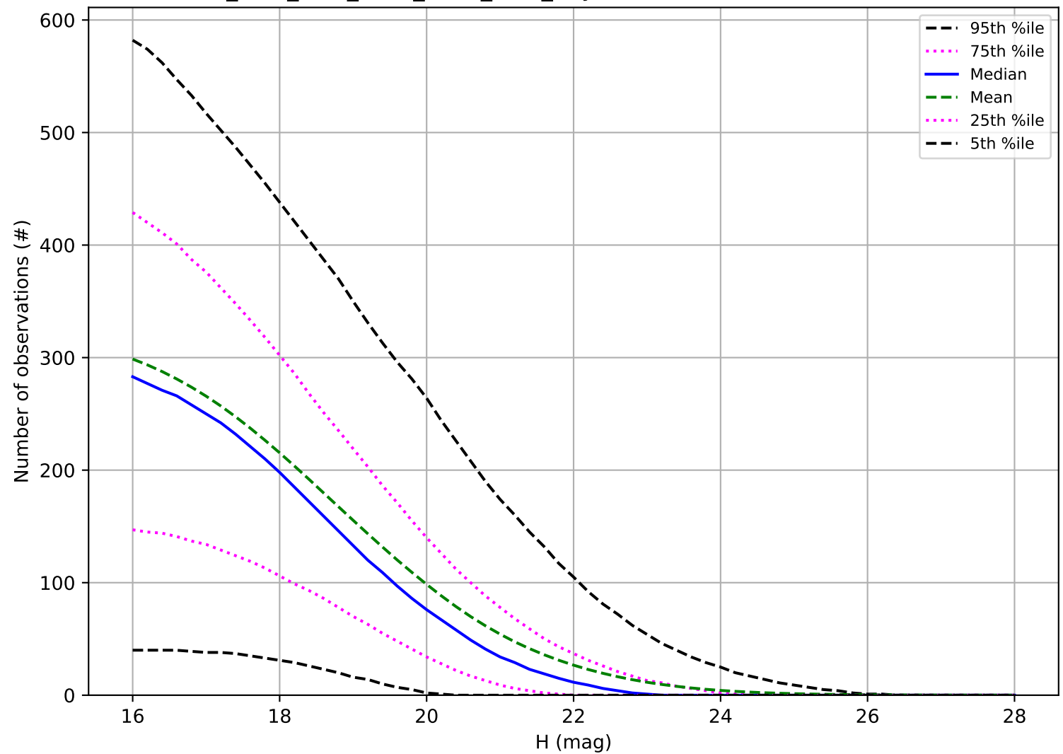
ddf_acor_sf15_lsf30_lsr50_v3.4_10yrs: Number of observations PHA
