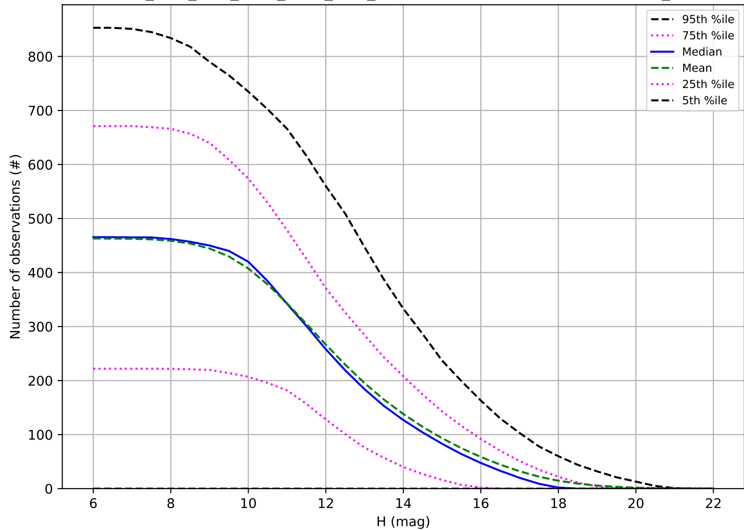
ddf_acor_sf15_lsf30_lsr50_v3.4_10yrs: Number of observations OCC_r5
