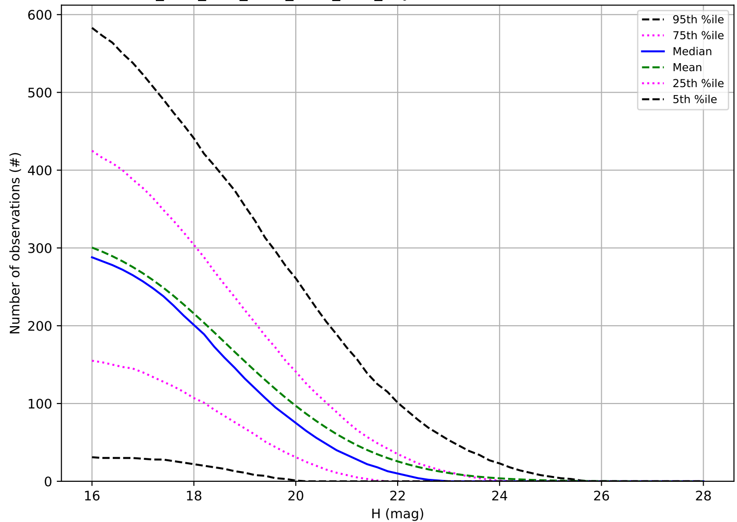
ddf_acor_sf15_lsf30_lsr50_v3.4_10yrs: Number of observations NEO
