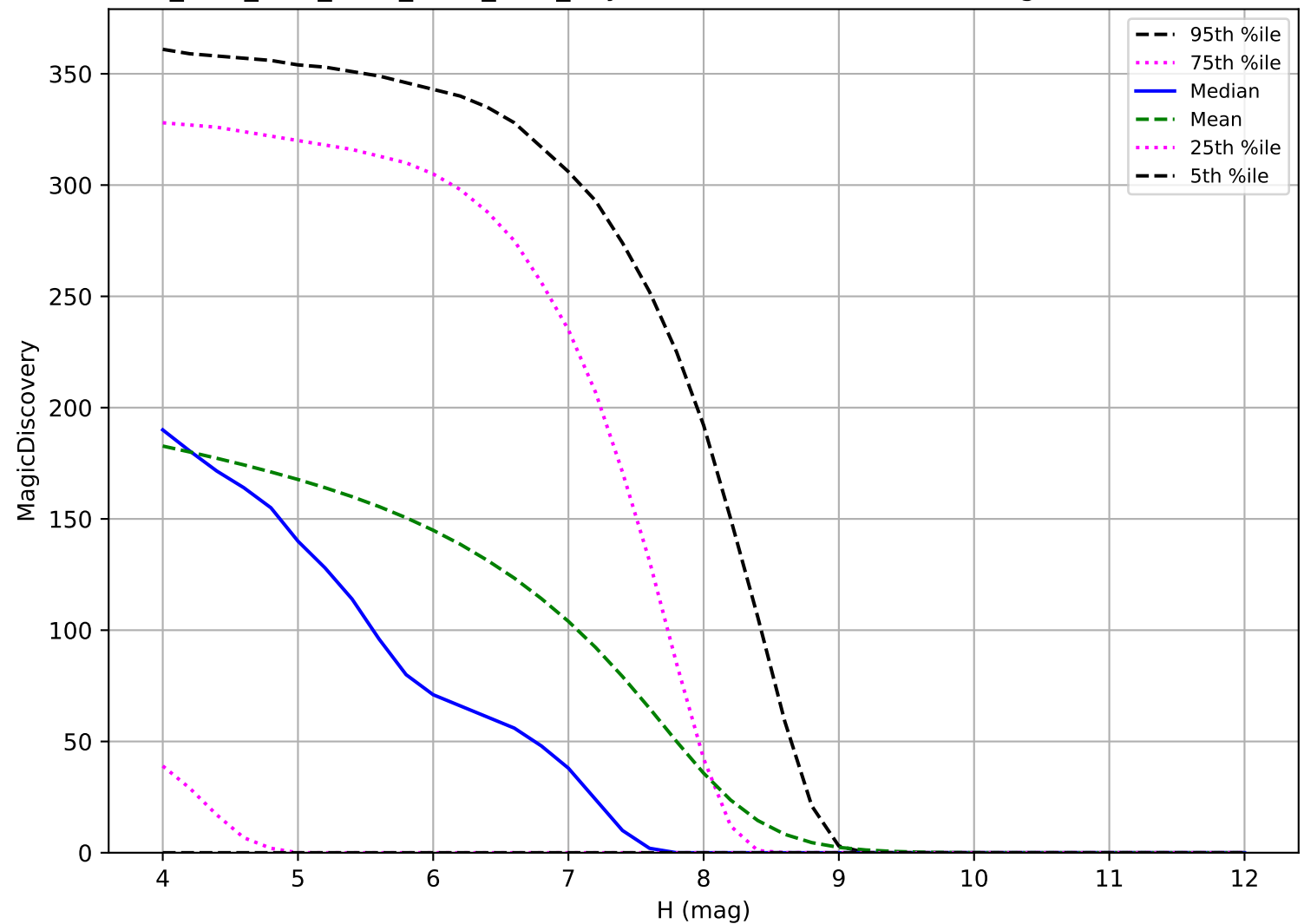
ddf_acor_sf15_lsf30_lsr50_v3.4_10yrs: TNO 6 detections in 60 nights detection loss
