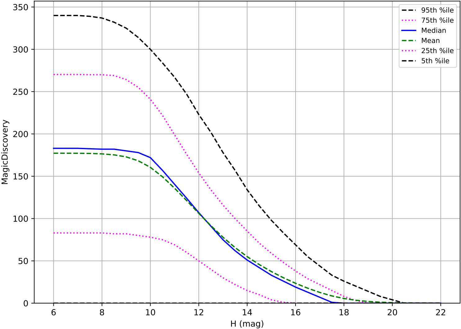
ddf_acor_sf15_lsf30_lsr50_v3.4_10yrs: OCC_r5 6 detections in 60 nights detection loss
