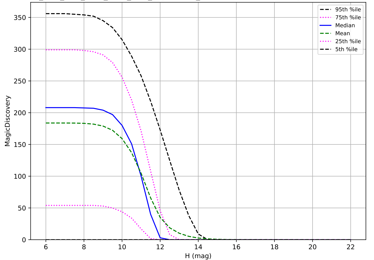
ddf_acor_sf15_lsf30_lsr50_v3.4_10yrs: OCC_r20 6 detections in 60 nights detection loss
