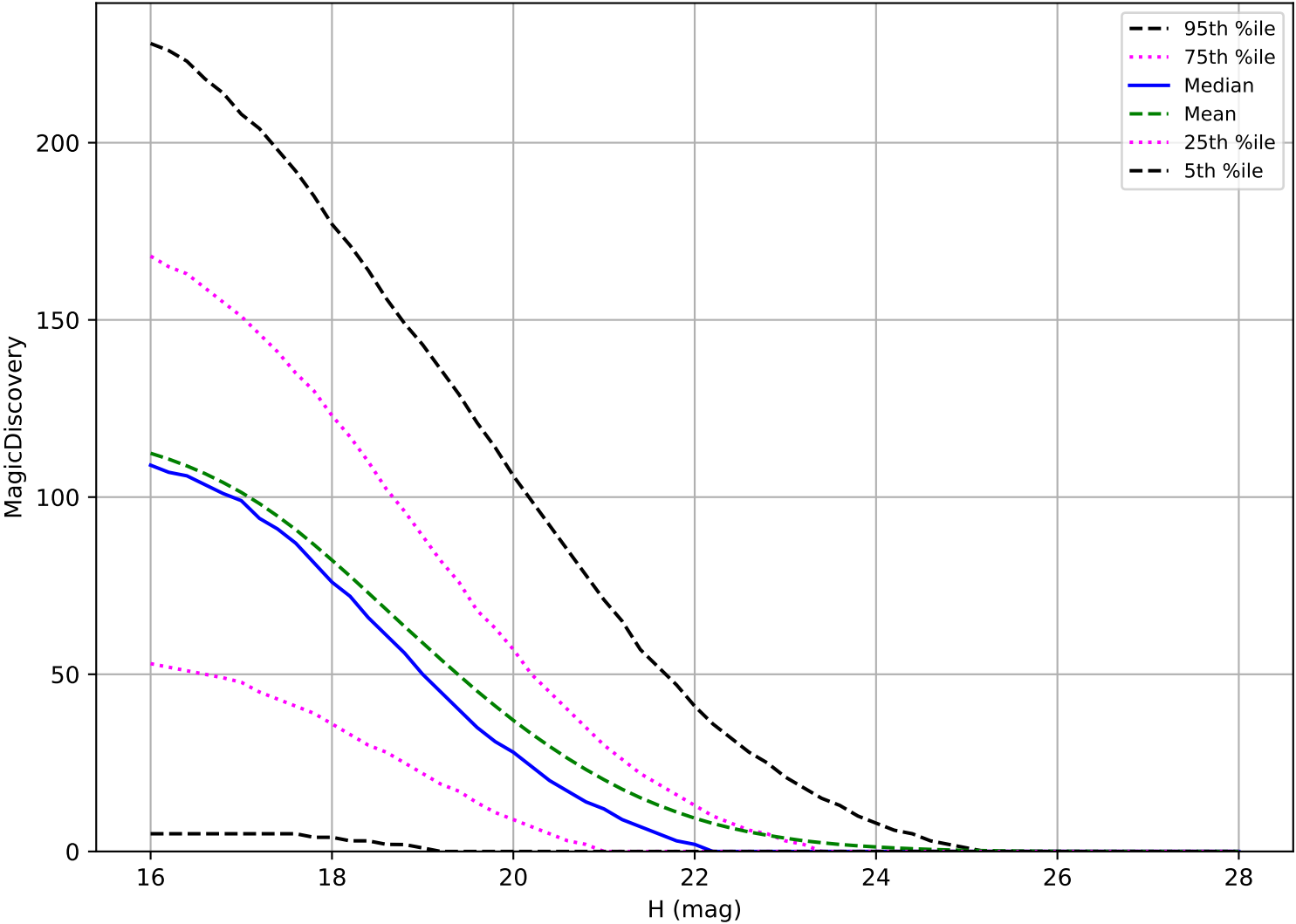
ddf_acor_sf15_lsf30_lsr50_v3.4_10yrs: NEO 6 detections in 60 nights detection loss
