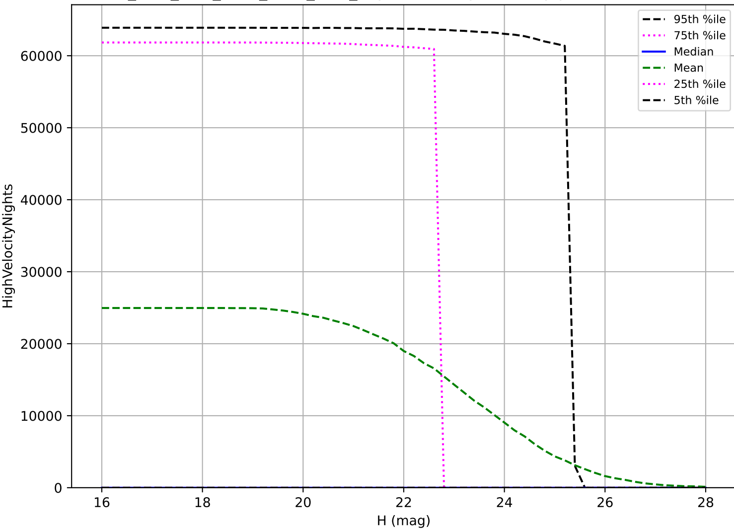
ddf_acor_sf15_lsf30_lsr50_v3.4_10yrs: PHA High velocity pair detection loss
