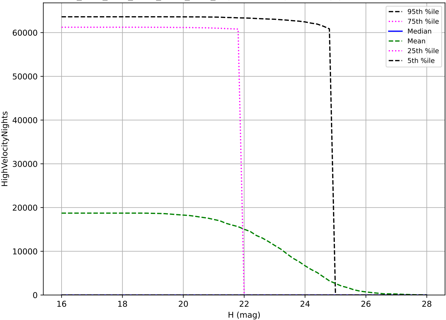
ddf_acor_sf15_lsf30_lsr50_v3.4_10yrs: NEO High velocity pair detection loss
