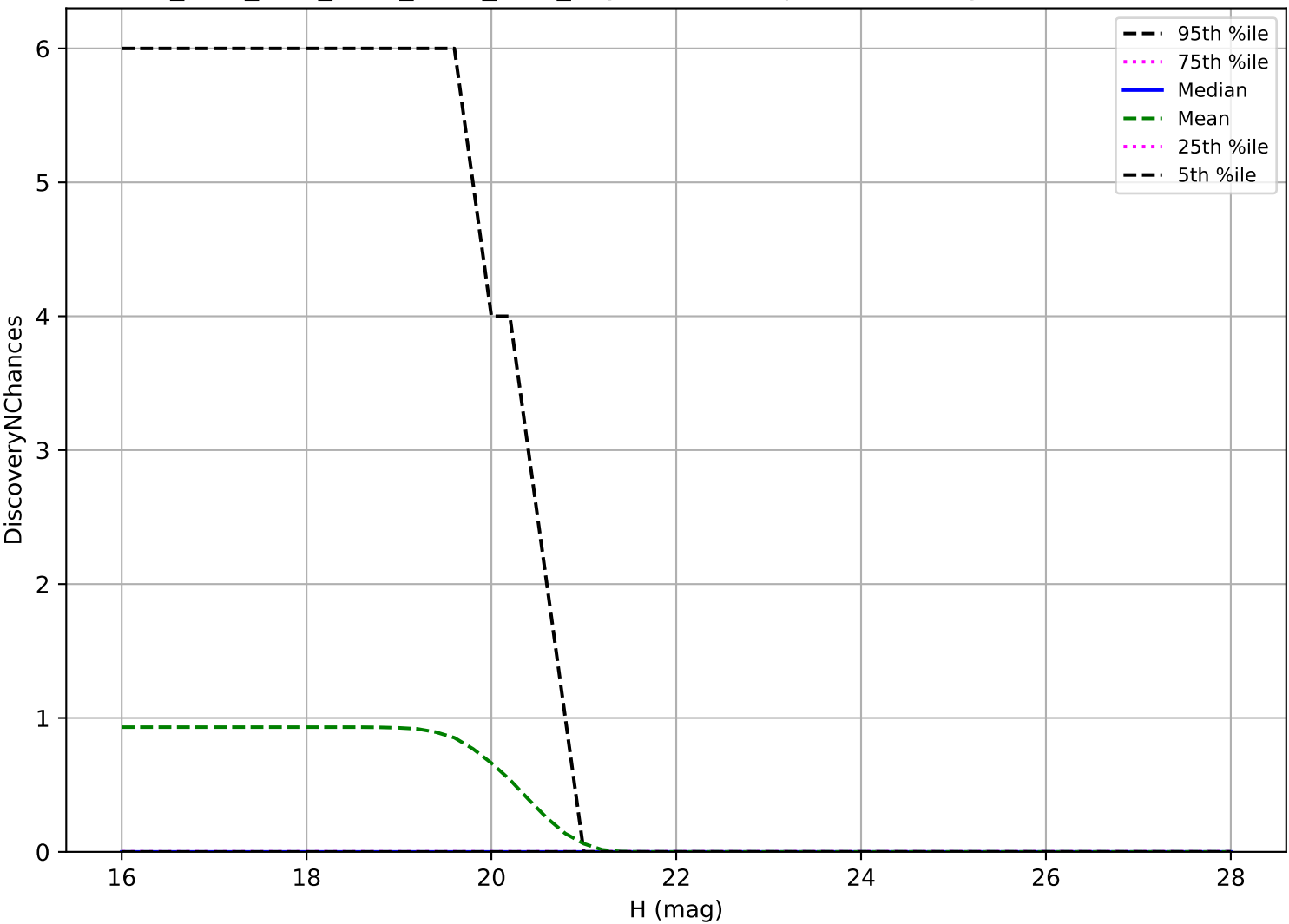
ddf_acor_sf15_lsf30_lsr50_v3.4_10yrs: Vatira 3 pairs in 15 nights detection loss
