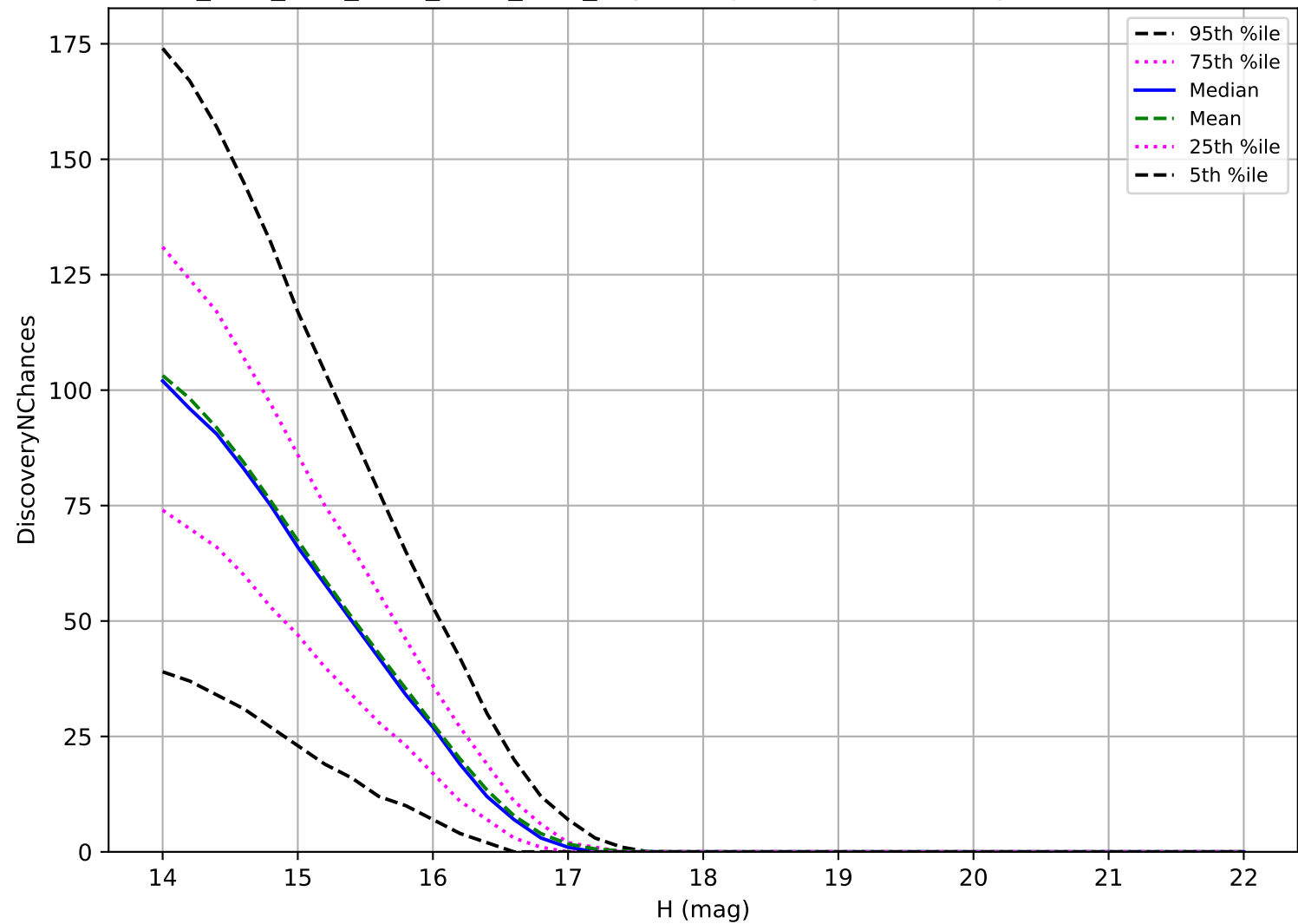
ddf_acor_sf15_lsf30_lsr50_v3.4_10yrs: Trojan 3 pairs in 15 nights detection loss
