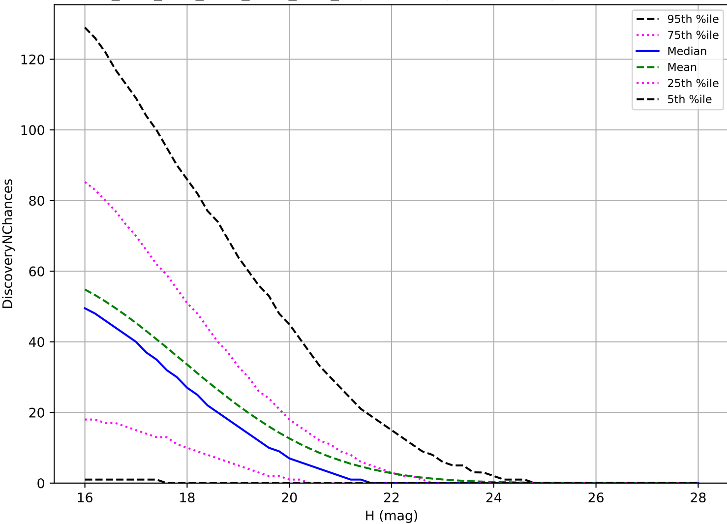
ddf_acor_sf15_lsf30_lsr50_v3.4_10yrs: PHA 3 pairs in 15 nights detection loss
