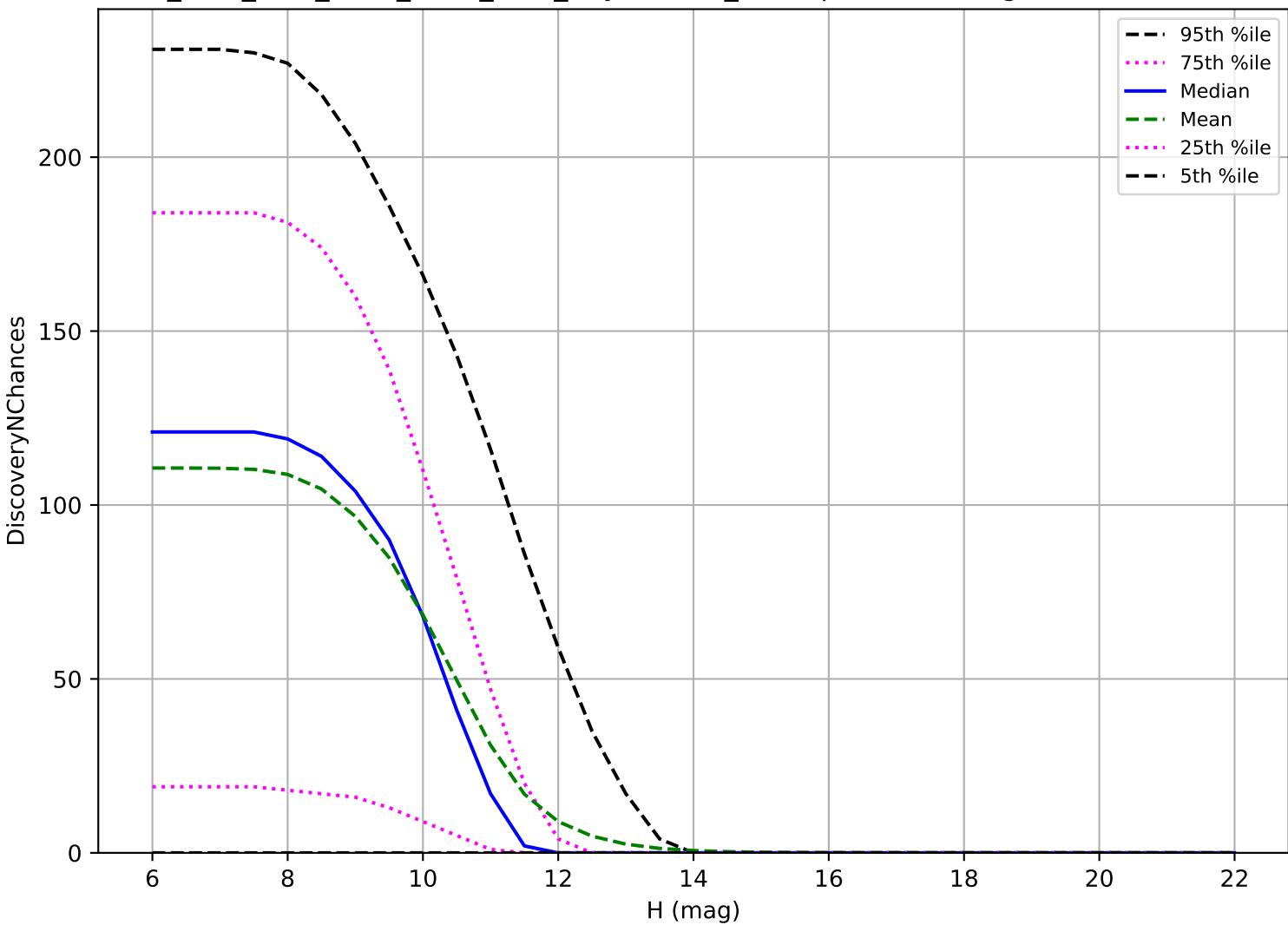
ddf_acor_sf15_lsf30_lsr50_v3.4_10yrs: OCC_r20 3 pairs in 15 nights detection loss
