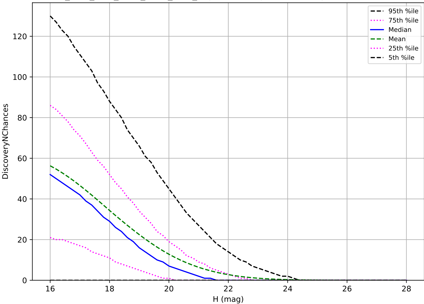
ddf_acor_sf15_lsf30_lsr50_v3.4_10yrs: NEO 3 pairs in 15 nights detection loss
