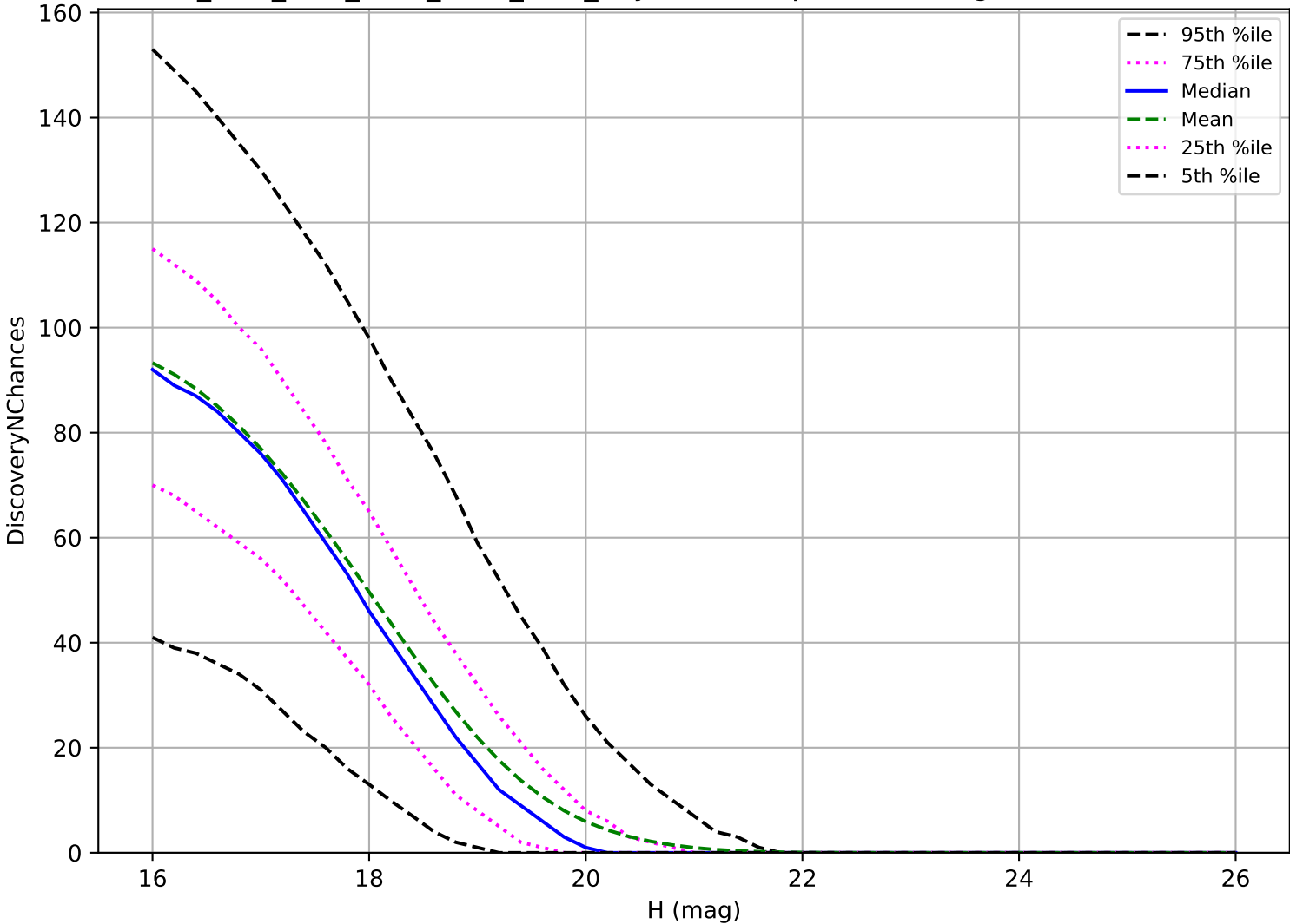
ddf_acor_sf15_lsf30_lsr50_v3.4_10yrs: MBA 3 pairs in 15 nights detection loss
