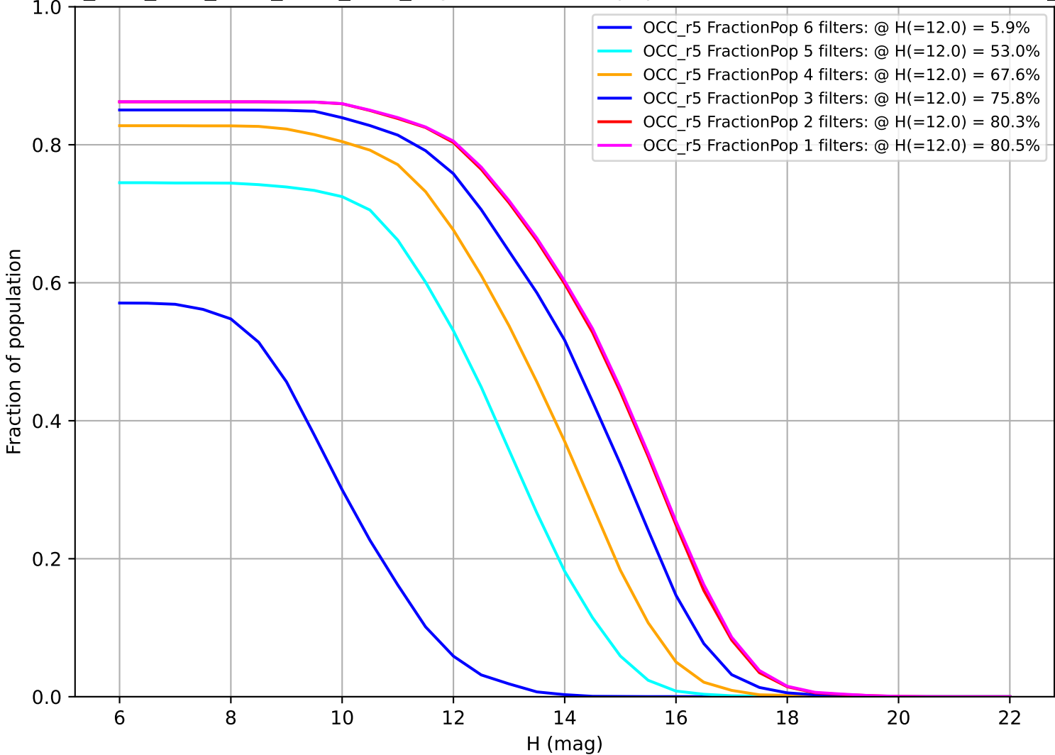
ddf_acor_sf15_lsf30_lsr50_v3.4_10yrs: Fraction of population with colors in X filters OCC_r5
