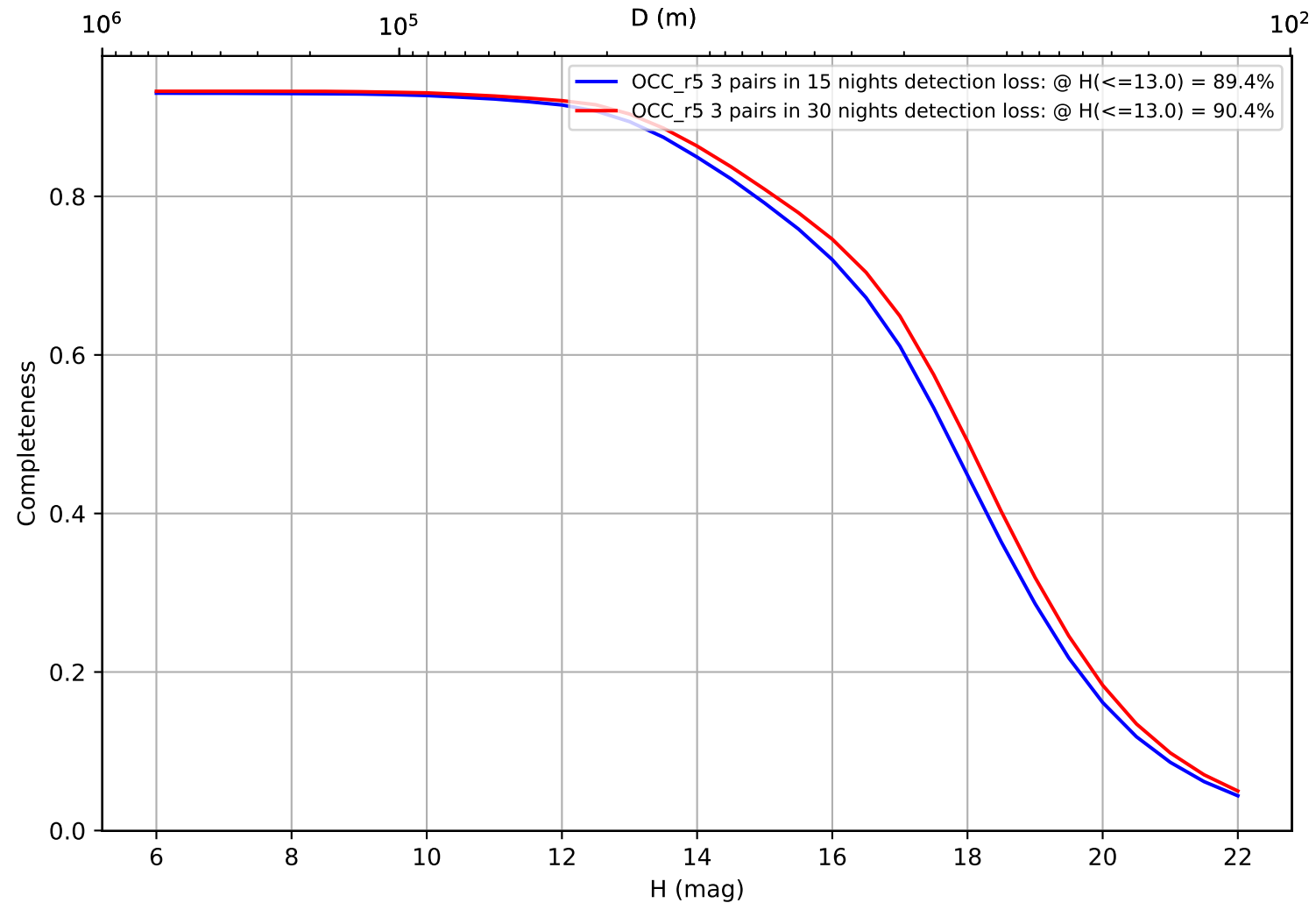
ddf_acor_sf15_lsf30_lsr50_v3.4_10yrs: CumulativeCompleteness
