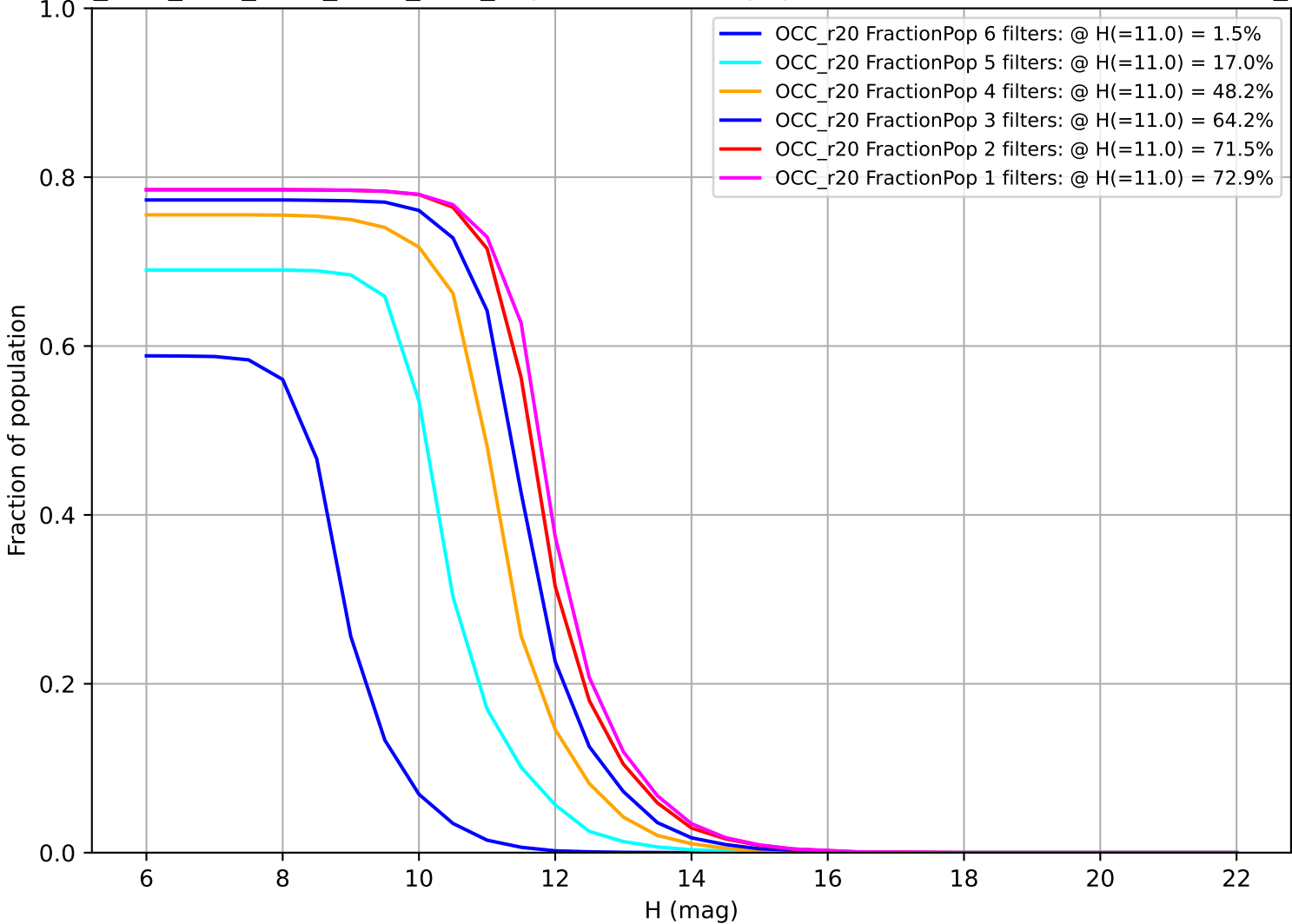
ddf_acor_sf15_lsf30_lsr50_v3.4_10yrs: Fraction of population with colors in X filters OCC_r20
