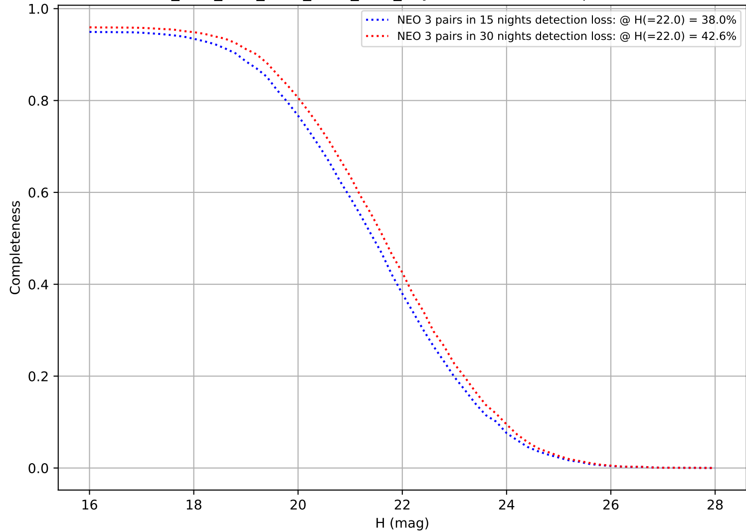
ddf_acor_sf15_lsf30_lsr50_v3.4_10yrs: DifferentialCompleteness
