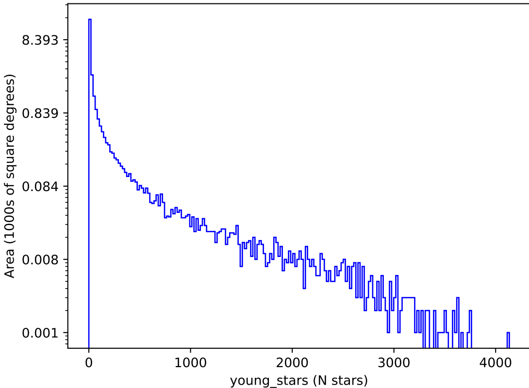
ddf_acor_sf15_lsf30_lsr50_v3.4_10yrs : young_stars
