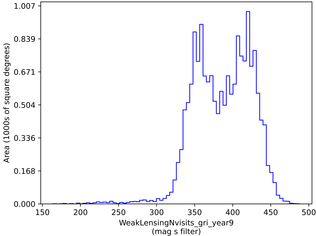
ddf_acor_sf15_lsf30_lsr50_v3.4_10yrs gri band non-DD: WeakLensingNvisits_gri_year9
