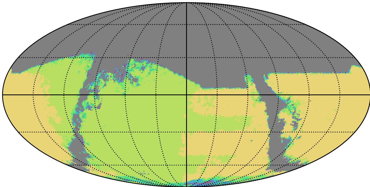
ddf_acor_sf15_lsf30_lsr50_v3.4_10yrs : TDC_campaign
