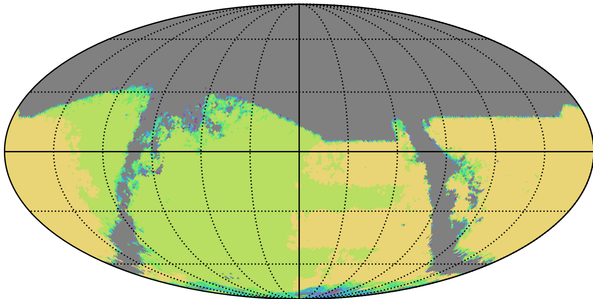
ddf_acor_sf15_lsf30_lsr50_v3.4_10yrs : TDC_campaign
