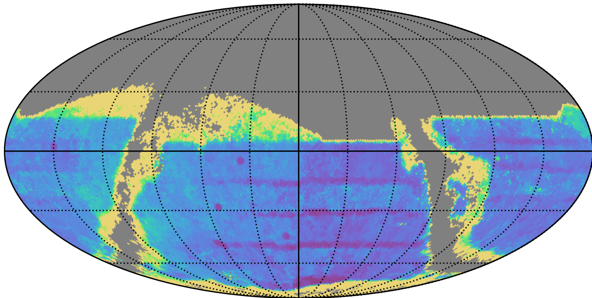
ddf_acor_sf15_lsf30_lsr50_v3.4_10yrs : TDC_accuracy
