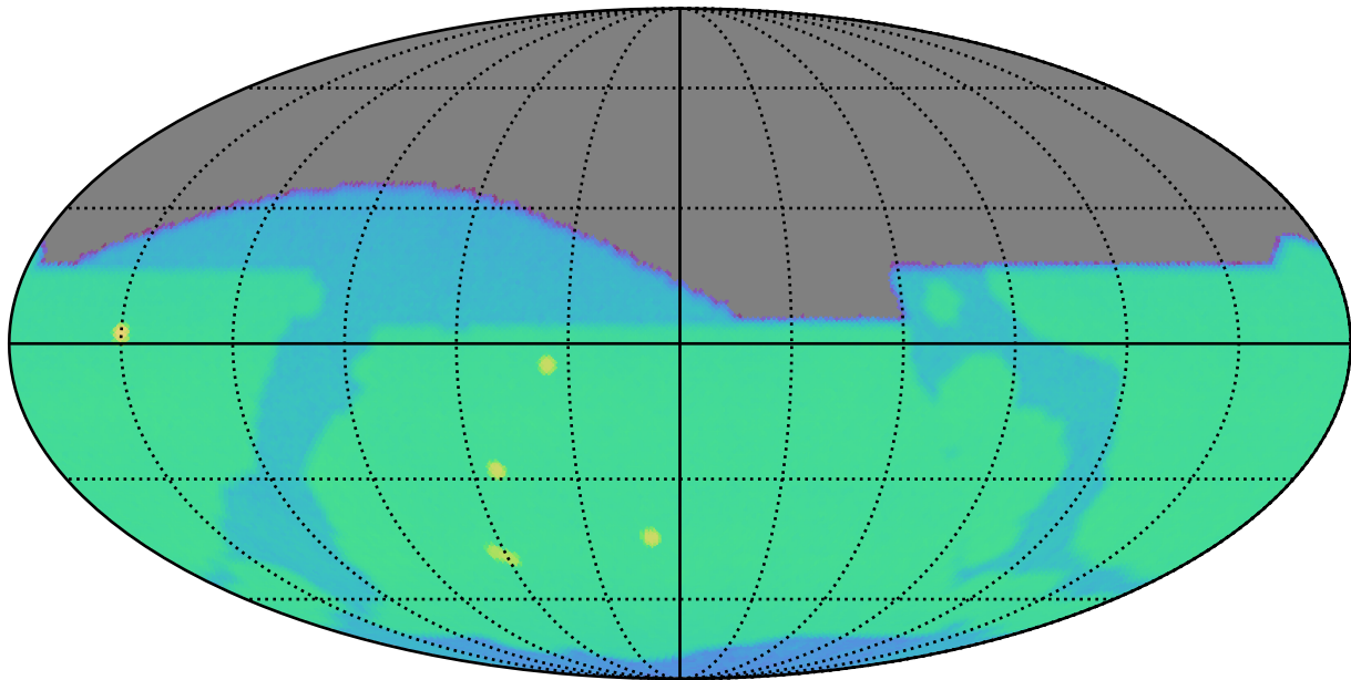
ddf_acor_sf15_lsf30_lsr50_v3.4_10yrs i: SurfaceBrightLimit
