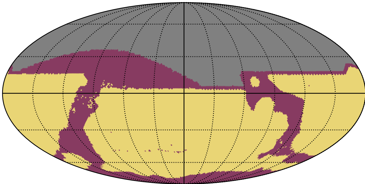
ddf_acor_sf15_lsf30_lsr50_v3.4_10yrs : RapidRevisits
