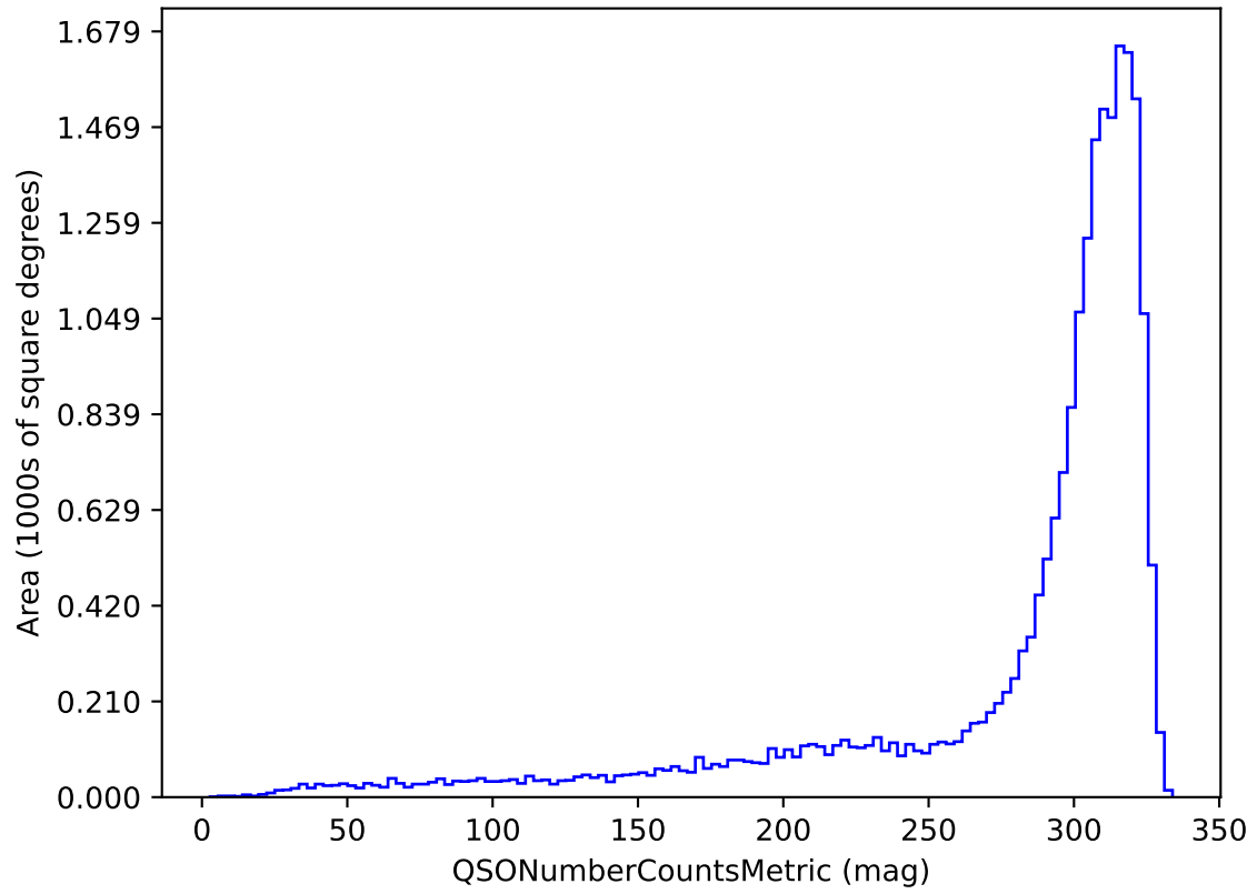
ddf_acor_sf15_lsf30_lsr50_v3.4_10yrs u band and non-DD: QSONumberCountsMetric
