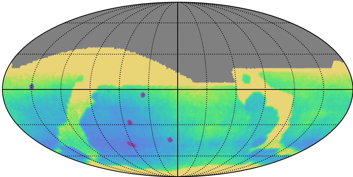
ddf_acor_sf15_lsf30_lsr50_v3.4_10yrs : Parallax Uncert @ 24.0
